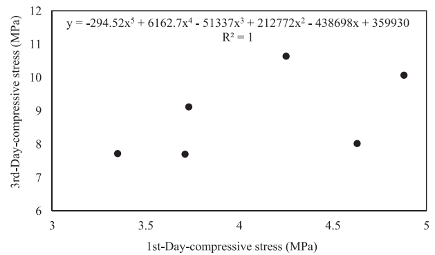
Fig. 15 – A fifth-degree equation between 1st-day-compressive stress and 3rd-day-compressive stress determined from the grout composites hardened.
