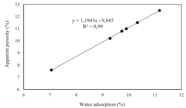
Fig. 8 – A linear model between apparent porosity and water adsorption of the hardened conventional grout composite and ecology-friendly grout composite doped flake of carbon and colloid flake of carbon.
